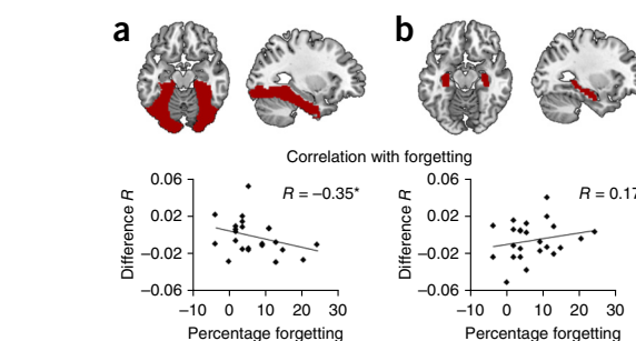
Figure 4 Correlation between item-specific competitor suppression and forgetting. (a,b) Across-participant correlations between cortical and behavioral suppression of competing memories are shown separately for ventral visual cortex (a) and hippocampus (b). The x axis in each graph shows our behavioral forgetting index on the delayed visual recognition memory test (forgetting of competitors relative to baseline items, with positive scores indicating more forgetting), and the y axis shows the overall cortical suppression of competitors during the selective recall task, calculated as the difference between reactivation of competitors and baseline items, averaged across all four repetitions. * P < 0.05 .
